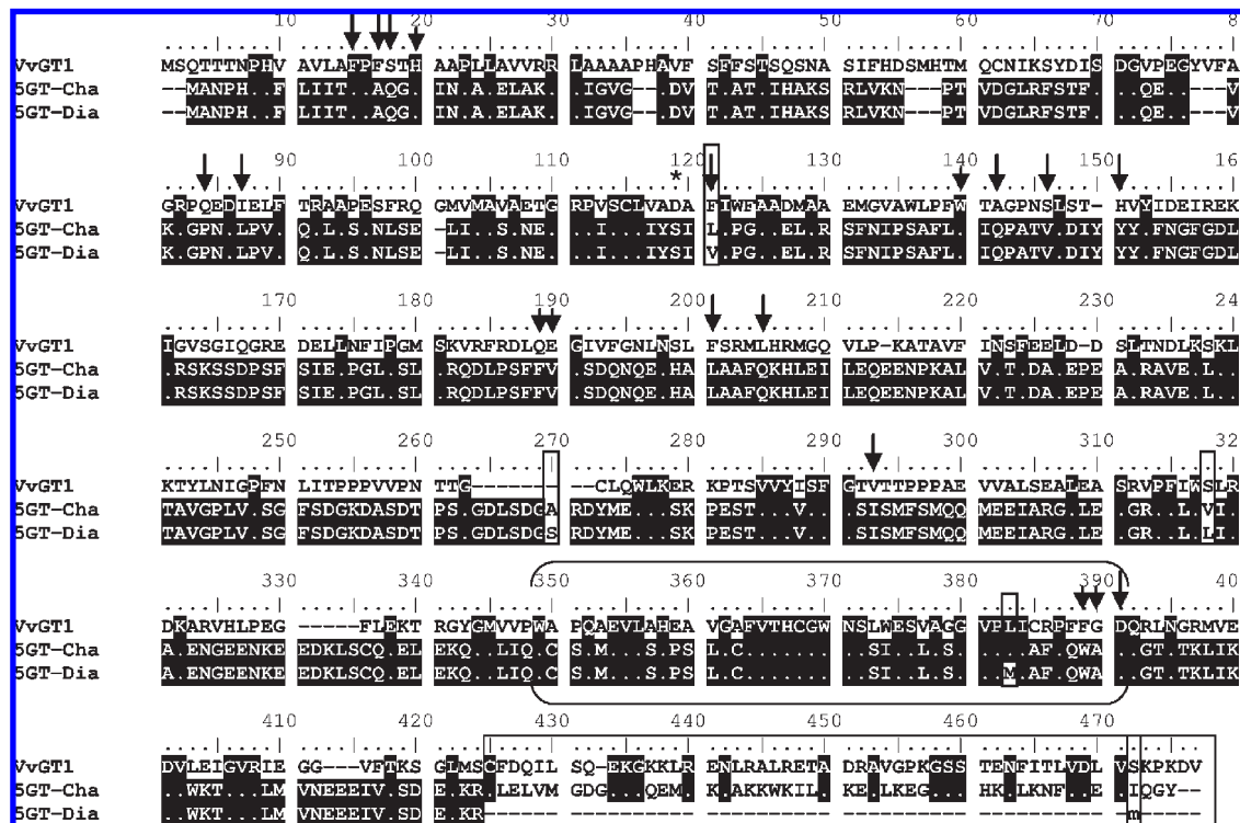
Figure 2. Protein sequence alignment of Vitis vinifera anthocyanidin 3- O -glucosyltransferase (VvGT1) and the functional 5- O -glucosyltransferase (5GT-Cha) and nonfunctional 5GT (5GT-Dia) from V. vinifera cv. Regent. The alignment was performed using ClustalX (31). Conserved amino acids are shaded, amino acids within 5 Å to quercetin in the protein model of VvGT1 are marked with an arrow, catalytically active amino acids are labeled with an asterisk, and amino acid exchanges in 5GT-Cha and 5GT-Dia are boxed. The positions of the amino acid exchanges in the original sequences are L110V, A259S, V307L, L372M, and I461M. The plant secondary product glucosyltransferase box, characteristic for GTs involved in natural product conjugation, is shown in parentheses.
